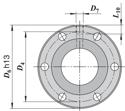
Flange type 1 6 holes at 60° ( d_0 < 40 mm)
