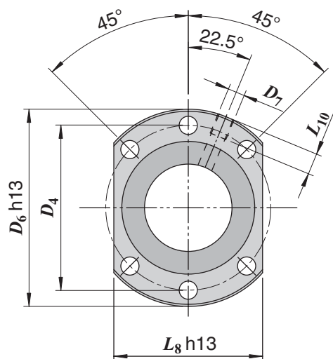
Flange type 1 (d_0 < 40 \text{ mm})
