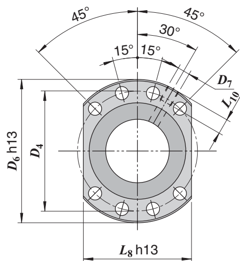
Flange type 2 (d_0 \geq 40 \text{ mm})
